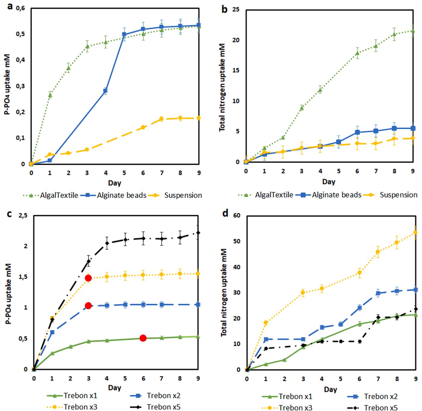
Fig. 3. – Phosphorus and total nitrogen uptake. 3a – Phosphorus uptake by microalgae in different cultivation methods. 3b – Nitrogen uptake by microalgae in different cultivation methods. 3c – Phosphorus uptake by AT at different concentrations of “Trebon” medium (red dots show the day when the P-PO 4 uptake reached 90% of the initial concentration in the medium). 3d – Nitrogen uptake by AT at different concentrations of “Trebon” medium.
